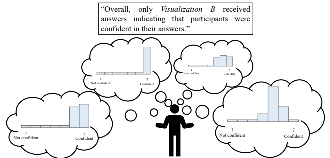
Figure 2: Describing Likert results verbally without giving the reader quantitative estimates of centrality and uncertainty can be ambiguous and may mislead the reader.
