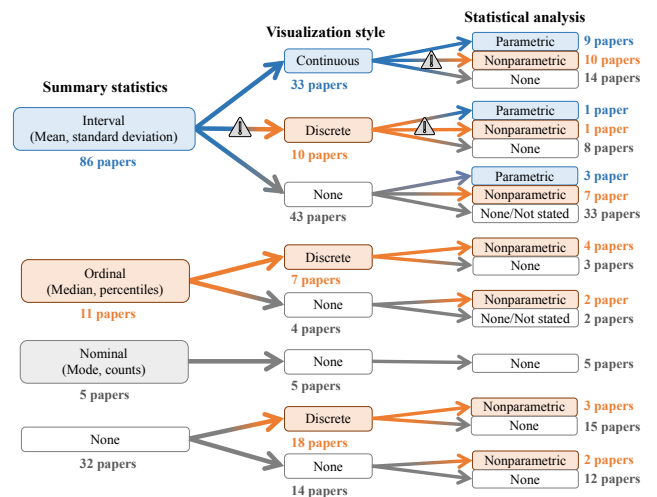
Figure 3: We recorded each paper’s decision to use intervalist or ordinalist interpretations for Likert scales at three points in reporting and analysis phases. Papers that used ordinal summary statistics maintained a consistent ordinalist interpretation, while several papers that began with interval summary statistics shifted to ordinalist interpretations later on in their analysis (indicated by \triangle icon).
